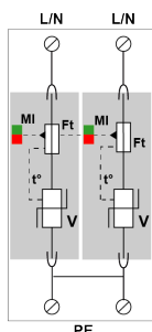
V: High-energy varistor Ft: Thermal fuse *: Thermal disconnection system MI: Disconnection indicator
