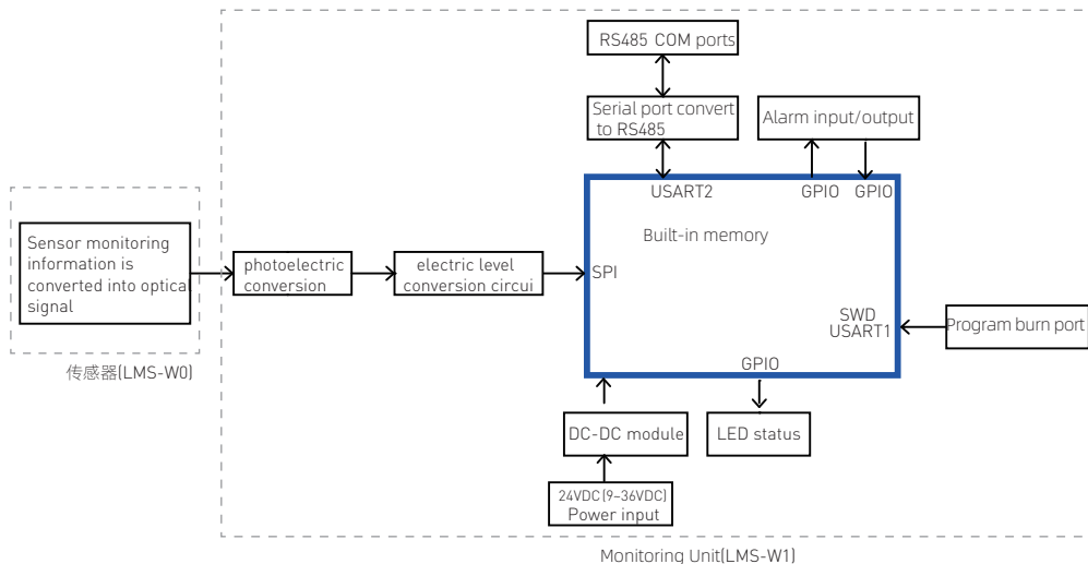
Figure 1. LMS-W system schematic
